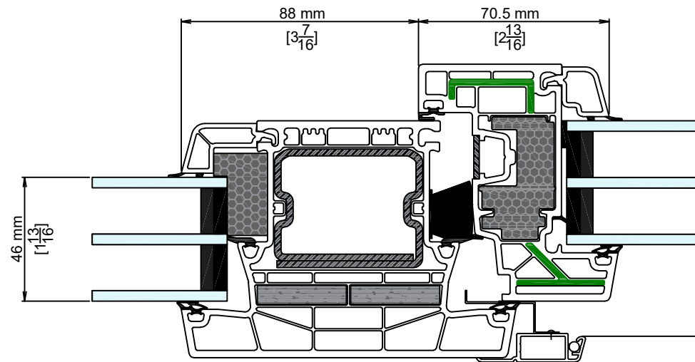
6 LARGE T-MULLION AT SASH
