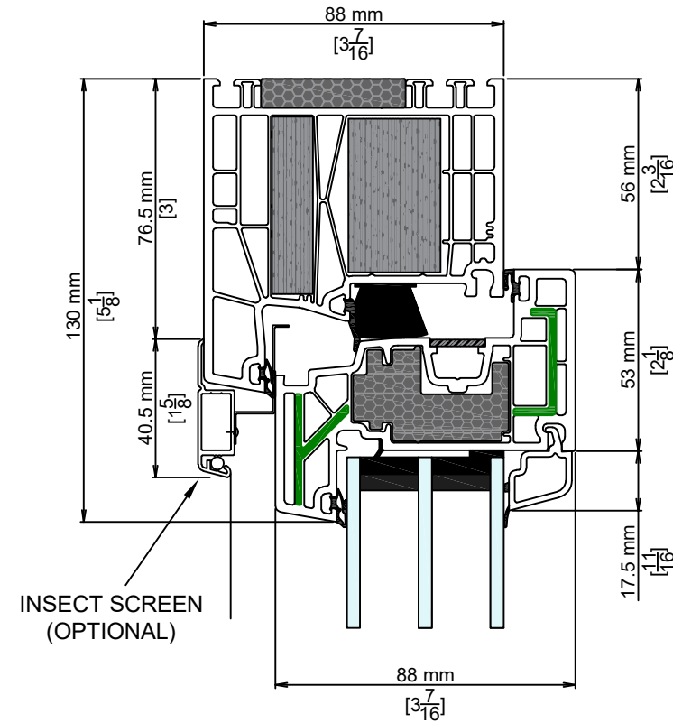
2 HEAD/JAMB/SILL AT SASH
