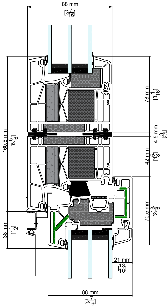
11 ZERO COUPLER AT FIXED/SASH
