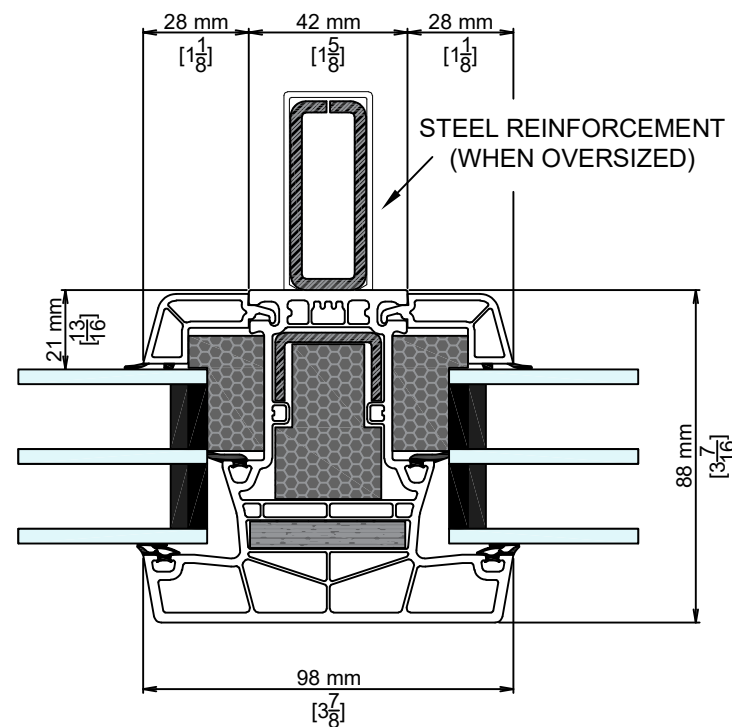
3 T-MULLION AT FIXED/FIXED
