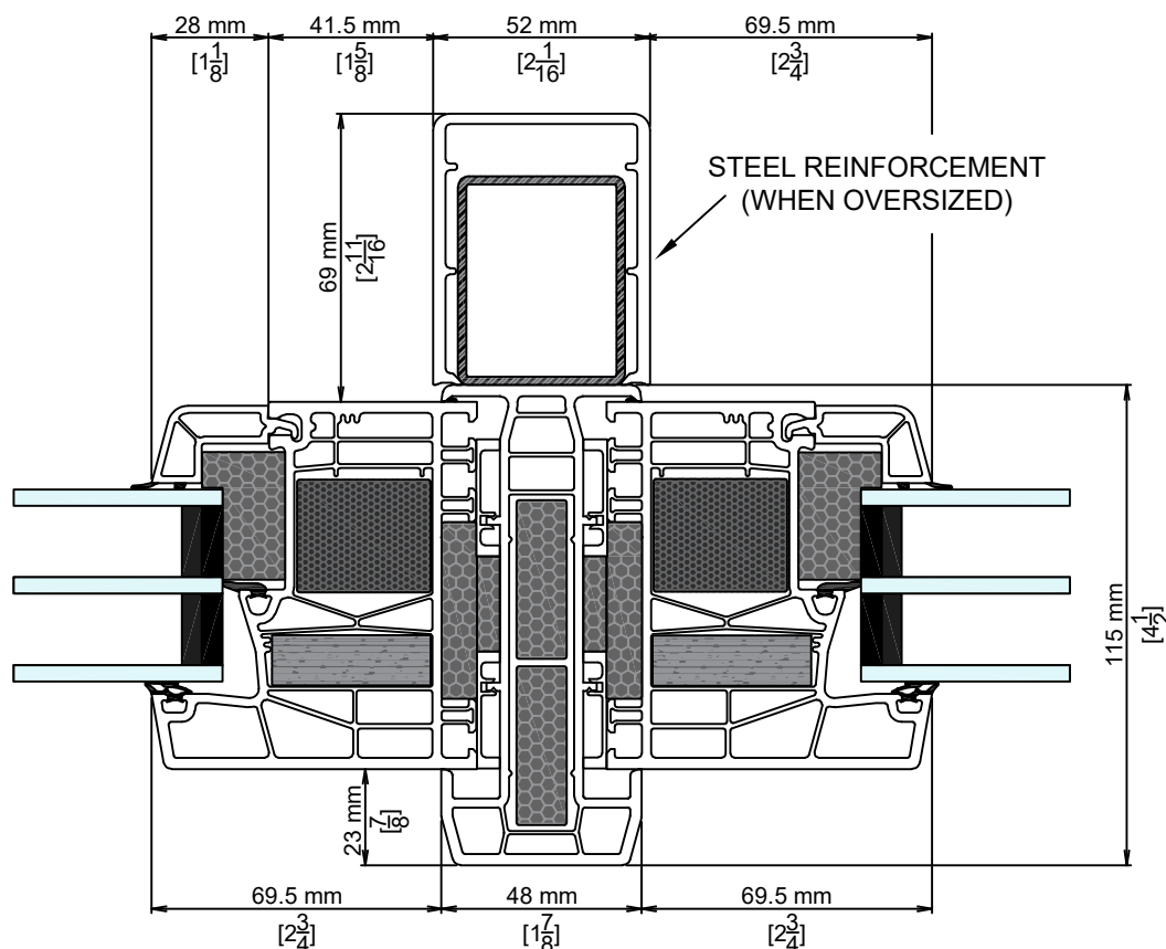
7 H-COUPLER AT FIXED/FIXED
