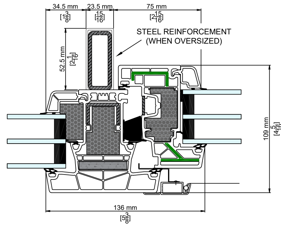
4 T-MULLION AT SASH/FIXED
