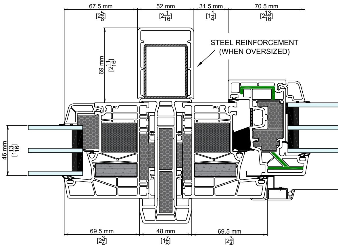
8 H-COUPLER AT FIXED/SASH
