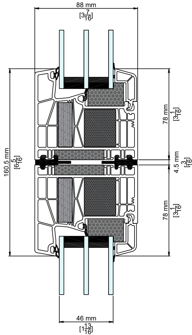
10 ZERO COUPLER AT FIXED/FIXED
