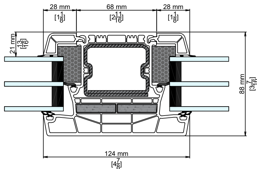
7 H-COUPLER AT FIXED/FIXED
